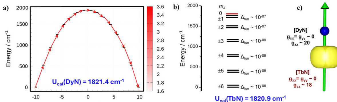
Fig. 4 Ab initio computed blockade barrier for (a) [DyN] and (b) [TbN] with the orientation of the g_{zz} axis (c). The yellow disk shows the beta-spin density.
