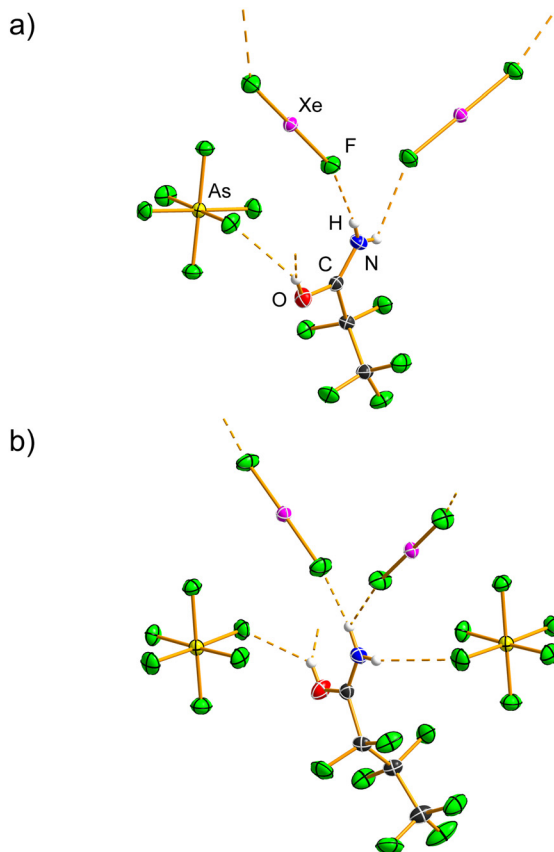
Fig. 7 Hydrogen bonds (dashed orange lines) in the crystal structures of the salt cocrystals (a) \text{C}_2\text{F}_5\text{C(OH)NH}_2[\text{AsF}_6]\cdot\text{XeF}_2 and (b) \text{C}_3\text{F}_7\text{C(OH)NH}_2[\text{AsF}_6]\cdot\text{XeF}_2 . The OH groups are bifurcated hydrogen-bond donors; however, two [\text{AsF}_6]^- anions have been omitted for clarity. Displacement ellipsoids are drawn at the 50% probability level, and hydrogen atoms are represented as spheres of arbitrary radius.
