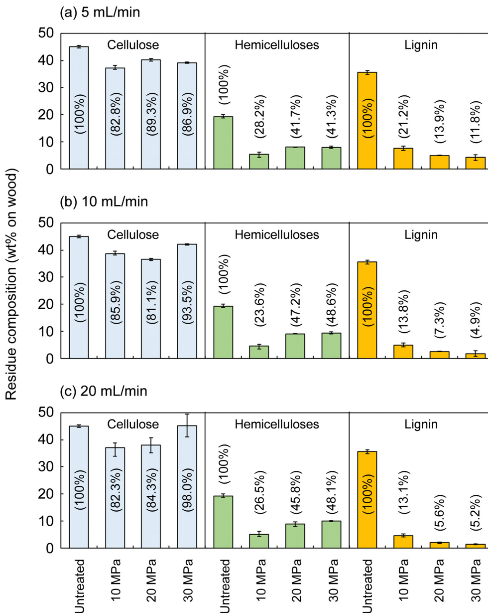
Fig. 2 Composition of the insoluble residue after the treatment of Japanese cedar wood with methanol/water (90/10, v/v) from room temperature to 270 °C (8 °C min -1 ) and at 270 °C for 30 min at various flow rates, (a) 5 mL min -1 , (b) 10 mL min -1 , and (c) 20 mL min -1 , and pressures (values in parentheses are percentages of the composition of untreated wood).
