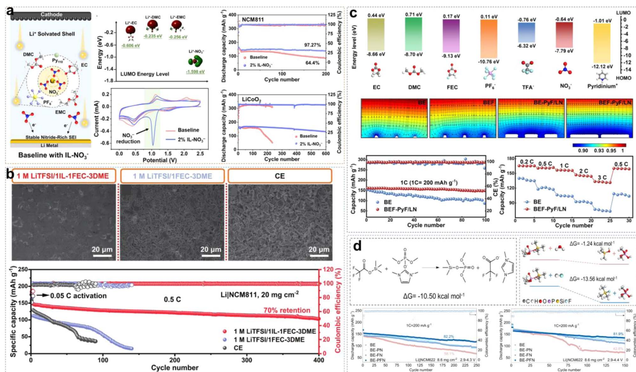
Fig. 14 (a) Solvation structure of 2\% \text{ IL-NO}_3^- electrolyte; LUMO energy level of \text{Li}^+ -complexes; CV curves of Li/Cu cells for the baseline electrolyte and 2\% \text{ IL-NO}_3^- electrolyte; cycling performance of Li/NCM811 and Li/LCO cells. Reprinted from ref. 128 with permission. Copyright 2023, Elsevier. (b) SEM images of the cycled LMA in different electrolytes and corresponding cycling performance of Li/NCM811 cells. Reprinted from ref. 129 with permission. Copyright 2022, Wiley. (c) Molecular orbital energies of solvents and additives calculated by DFT; finite element analysis of Li deposition morphology simulated by COMSOL Multiphysics; cycling and rate performance of Li/LCO cells. Reprinted from ref. 130 with permission. Copyright 2022, Elsevier. (d) The reaction between DIDP and TMSF and the reaction paths of DTSP and \text{H}_2\text{O}/\text{HF} ; long-term cycling performance in Li/NCM622 cells. Reprinted from ref. 131 with permission. Copyright 2024, Wiley.
