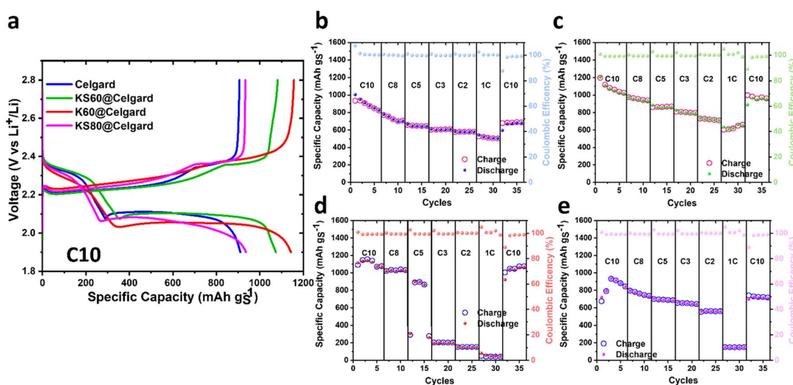
Fig. 3 (a) GCD profiles recorded at C10 of the LSBs (sulphur loading: \sim 2\text{ mg}_\text{s}\text{ cm}^{-2} ; E/S ratio: 15\text{ }\mu\text{L mg}_\text{s}^{-1} , electrode geometric area: 1.54\text{ cm}^2 ) containing pristine Celgard, KS60@Celgard, K60@Celgard and KS80@Celgard separators. Rate performance from C10 to 1C of the Li–S batteries containing (b) pristine Celgard, (c) KS60@Celgard, (d) K60@Celgard and (e) KS80@Celgard separators.
