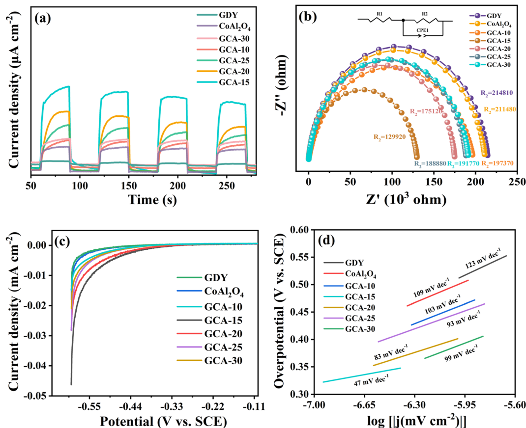
Fig. 12 (a) Transient photocurrent responses for GDY, \text{CoAl}_2\text{O}_4 and GCA-X; (b) EIS of GDY, \text{CoAl}_2\text{O}_4 and GCA-X; (c) LSV curves of GDY, \text{CoAl}_2\text{O}_4 and GCA-X and (d) the corresponding Tafel plots for GDY, \text{CoAl}_2\text{O}_4 and GCA-X.
