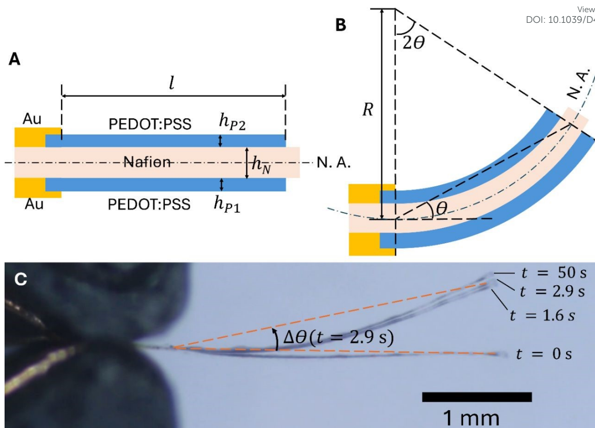
Fig. 3. (A) Schematic showing the dimensional parameters for an AJP actuator in the neutral position before bending. The dashdotted line labelled ‘N. A.’ indicates the neutral axis. (B) Schematic of an AJP actuator under actuation, showing the relationship among bending angle \theta , actuator length l , and radius of curvature R . (C) Overlaid snapshots showing actuation of an actuator with 5.6 \mu\text{m} Nafion electrolyte thickness and 1.1 \mu\text{m} PEDOT:PSS thickness, under an applied DC voltage of 0.8 \text{ V} . The actuator achieves 90% maximum charge transfer in 1.6 \text{ s} and 90% maximum deflection in 2.9 \text{ s} .
