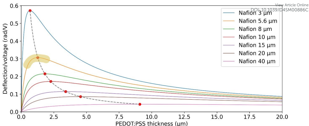
Fig. 5. Predicted deflection-to-voltage ratio against PEDOT:PSS electrode thickness, for different Nafion electrolyte thicknesses. The dashed line traces the peak of the curves. The highlighted region shows approximately the range where the actuation tests of actuators with different PEDOT:PSS thicknesses ( Fig. 4B ) were conducted.
