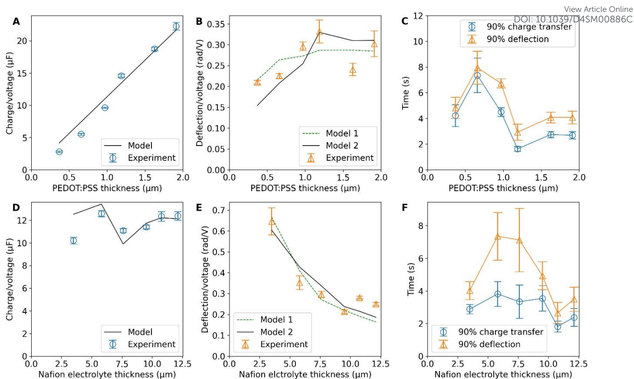
Fig. 4. (A) Charge-to-voltage ratio ( \frac{\Delta Q}{V_{appl}} ), (B) deflection-to-voltage ratio ( \frac{\theta}{V_{appl}} ) and (C) time taken to reach 90% charging and 90% deflection for samples with different PEDOT:PSS electrode thicknesses (harmonic mean electrode thicknesses). (D) Charge-to-voltage ratio ( \frac{\Delta Q}{V_{appl}} ), (E) deflection-to-voltage ratio ( \frac{\theta}{V_{appl}} ) and (F) time taken to reach 90% charging and 90% deflection for samples with different PEDOT:PSS electrode thicknesses. The modelling results in (A), (B), (D), and (E) are discrete points with the same x-values as the experiment data but are connected with lines for visualisation. The data points in (C) and (F) are also connected with lines for visualisation. Error bars for all plots indicate standard deviation of data points with Bessel's correction. Note that while the models in (B) and (E) can be applied to asymmetric trilayers, which exhibit unequal forward and backward deflection-to-voltage ratios, the differences in our data are minimal as the actuators are largely symmetrical. Therefore, the forward and backward deflection data have been combined for each actuator due to the difficulty in consistently identifying which side is which.
