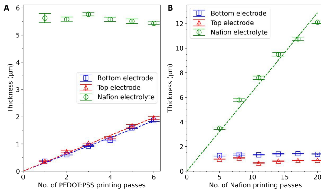
Fig. 2. Thicknesses of PEDOT:PSS and Nafion against number of printing passes in (A) 6 actuator samples with PEDOT:PSS thickness variation and (B) 6 actuator samples with Nafion thickness variation. The error bars indicate standard deviation of results from 4 profilometry scans with Bessel's correction. The dashed lines are linear fits of the data points through the origin.
