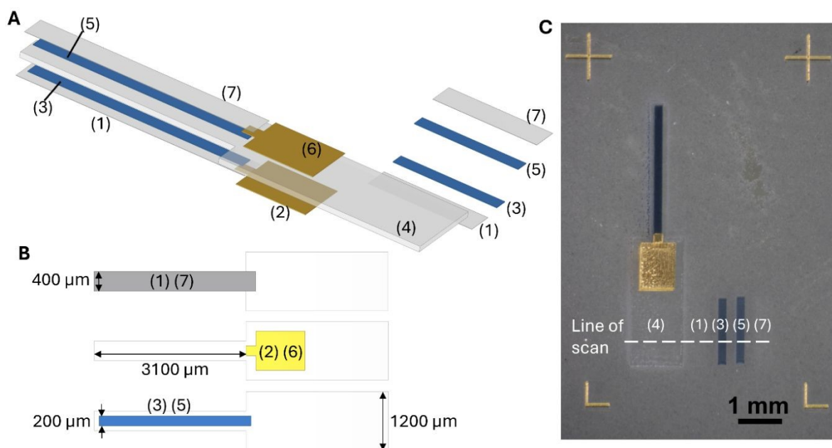
Fig. 1. (A) Exploded diagram showing multilayer structure of AJP actuator and sequence of printing. The rectangular pieces on the right are thickness test samples. Layer 1: Nafion bottom encapsulation layer; Layer 2: Au bottom layer; Layer 3: PEDOT:PSS bottom layer; Layer 4: Nafion electrolyte layer; Layer 5: PEDOT:PSS top layer; Layer 6: Au top layer; Layer 7: Nafion top encapsulation layer. The thickness of each layer is exaggerated ~10 times in comparison to length and width. (B) Diagram showing position of Nafion encapsulation layers (Layers 1 and 7), Au layers (Layers 2 and 6) and PEDOT:PSS layers (Layers 3 and 5) relative to the Nafion electrolyte layer (Layer 4). (C) Optical image of a printed actuator along with thickness test samples. The fiducial markers at the corners are printed to ensure accurate alignment of different layers. The thickness of Layers 4, 1, 3, 5, and 7 are obtained by a profilometer scanning along the direction shown by the dashed line.
