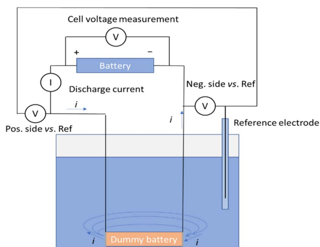
Fig. 2 Schematic of the measurement system.
