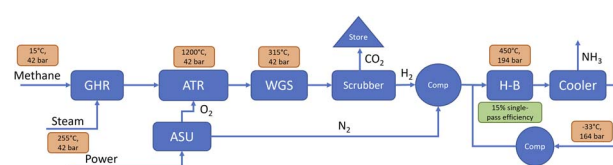
Fig. 3 Simplified process drawing of the ATR-based blue ammonia synthesis process. "GHR" is the gas heated reformer, "ATR" the auto-thermal reformer, "WGS" is the water gas shift reactor, "H-B" the Haber–Bosch reactor, "ASU" the air separation unit, and "Comp" are compressors.
