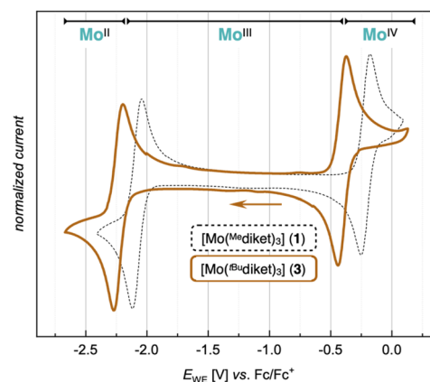
Fig. 3 CV of [\text{Mo}(t\text{Bu}_2\text{diket})_3] ( 3 ) (1 mM, solid line) and [\text{Mo}^{\text{Me}}(\text{Me}_2\text{diket})_3] ( 1 ) (1 mM, dashed line) in \text{TBAPF}_6/\text{MeCN} (0.1 M) at a scan rate of \nu = 100 \text{ mV s}^{-1} .
