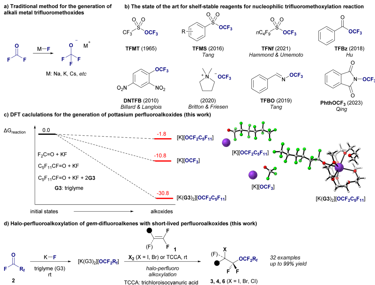
Fig. 1 Background and strategy of nucleophilic perfluoroalkoxylation. (a) Traditional method for the preparation of alkali metal trifluoromethoxides. (b) Shelf-stable reagents for nucleophilic trifluoromethoxylation. (c) DFT-calculated reaction Gibbs free energy B3LYP-D3/6-311+G(d,p) in ether (SMD), in \text{kcal mol}^{-1} for the reactions of KF with \text{F}_2\text{C}=\text{O} ( -10.8 \text{ kcal mol}^{-1} ), \text{C}_5\text{F}_{11}\text{CF}=\text{O} ( -1.8 \text{ kcal mol}^{-1} ) and \text{C}_5\text{F}_{11}\text{CF}=\text{O} with triglyme ( -30.8 \text{ kcal mol}^{-1} ) (this work). (d) Halo-perfluoroalkoxylation of olefins (this work).
