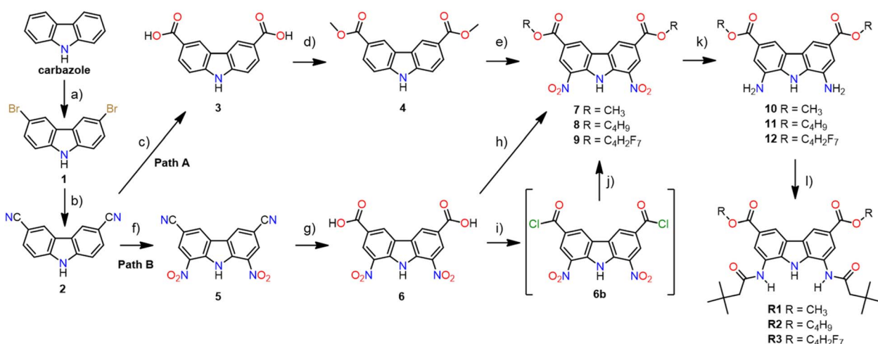
Scheme 1 The synthesis of receptors R1–R3 : (a) NBS, DMF, –5 °C, 1 h, 57%; (b) Zn(CN) 2 , dpf, Zn, Zn(OAc) 2 , Pd 2 (dba) 3 (cat.), DMF, H 2 O, 110 °C, 72 h, 97%; (c) 2 M NaOH, CuI, 100 °C, 24 h, 98%; (d) MeOH, 95% H 2 SO 4 (cat.) reflux, 24 h, 90%; (e) 65% HNO 3 , 95% H 2 SO 4 (cat.), 0 °C, 0.5 h, 26%; (f) 100% HNO 3 , Ac 2 O, AcOH, 110 °C, 49%; (g) H 2 O, AcOH, 95% H 2 SO 4 (cat.), 110 °C, 16 h, 88%; (h) MeOH, 95% H 2 SO 4 (cat.), reflux, 24 h, 78% for 7 or BuOH, 95% H 2 SO 4 (cat.), 135 °C, 20 h, 90% for 8 ; (i) SOCl 2 , DMF, 60 °C, 4 h; (j) 2,2,3,3,4,4,4-heptafluorobutyl alcohol, DCM, TEA, 85%; (k) H 2 , 0.3 bar, 10% Pd/C (cat.), AN, RT, 7 h for 10 or 5 h for 11 & 12 , 77% for 10 , 89% for 11 , 87% for 12 ; (l) t -butylacetyl chloride, TEA, THF, RT, 1 h, 66% for R1 , 56% for R2 , 73% for R3 .
