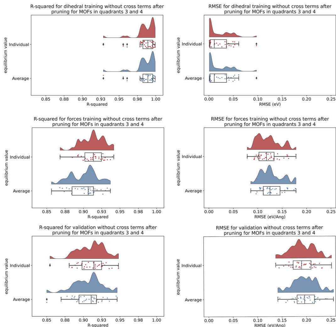
Fig. 28 Raincloud plots of R -squared (left panels) and RMSE (right panels) for rotatable dihedrals training (top panels), forces training (central panels), and validation (bottom panels) for MOFs in quadrants 3 and 4 without cross terms and after pruning. The red distributions represent the values for individual equilibrium values, while the blue distributions represent the values for average equilibrium values.
