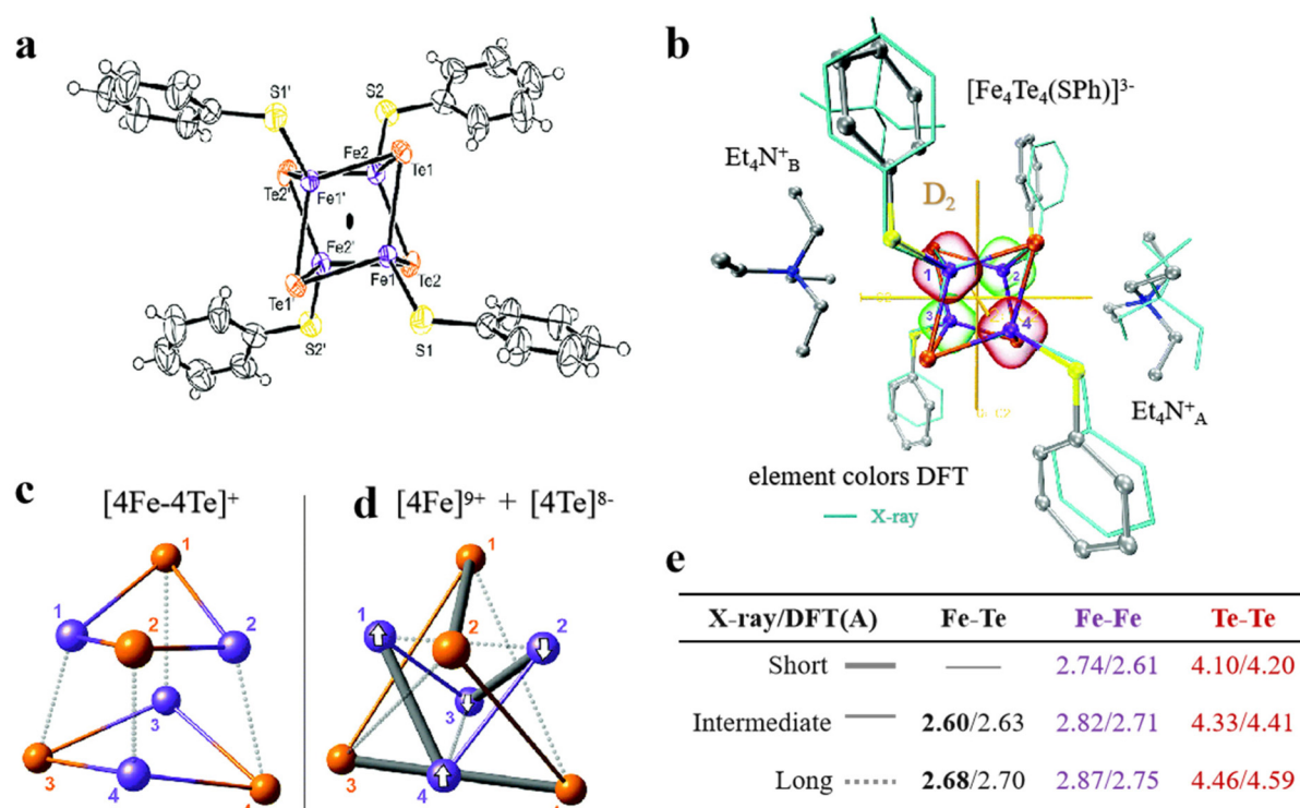
Fig. 9 Artificial Fe-S clusters based on Te element doping. (a) The structure of [\text{Fe}_4\text{Te}_4] cluster. (b) D_2 -symmetric [\text{Fe}_4\text{Te}_4] clusters obtained by X-ray and DFT optimization. (c and d) The bonding interactions and (e) bond length information of [\text{Fe}_4\text{Te}_4] cluster cores. Reproduced with permission from ref. 98. Copyright 2019, Royal Society of Chemistry.
