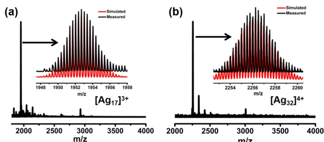
Fig. 1 (a) Positive-ion mode ESI-MS of Ag 17 in CH 3 OH. (Inset) Measured (black line) and simulated (red line) isotopic distribution patterns of the molecular ion peak. (b) Positive-ion mode ESI-MS of Ag 32 in CH 3 OH. (Inset) Measured (black line) and simulated (red line) isotopic distribution patterns of the molecular ion peak.
