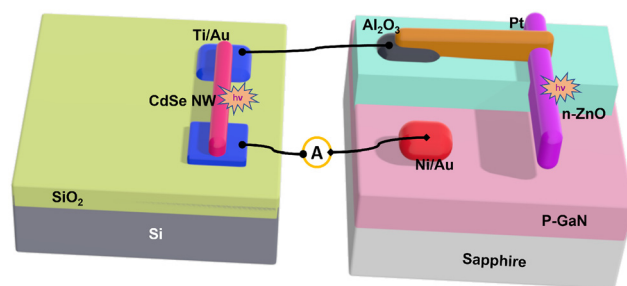
Fig. 4 Schematic of a CdSe NW-based photodetector utilizing a ZnO/p-GaN-based energy harvesting unit. 45
