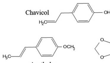
Anethole
