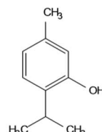
Thymol
