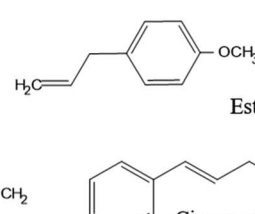
Cinnamyl alcohol
