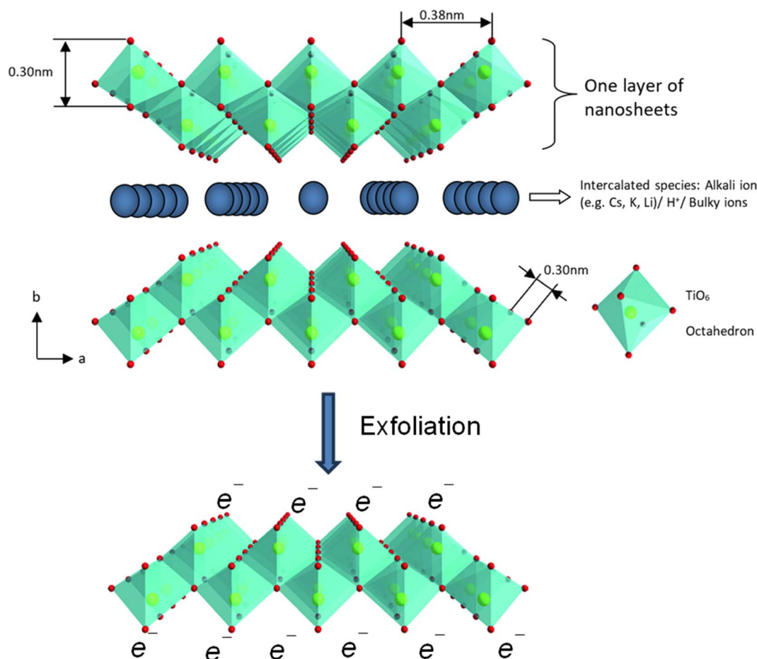
Fig. 11 The polyhedral representation of the crystal structure of layered lepidocrocite-like titania nanosheets viewed down along the c -axis and mono-layer titanate nanosheets after exfoliation. Adapted from ref. 88 with permission from the Royal Society of Chemistry.
