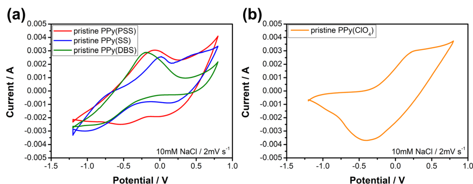
Fig. 3 Cyclic voltammograms of (a) positive electrode materials, PPy(PSS), PPy(SS), and PPy(DBS) and (b) a negative electrode material, PPy(ClO 4 ) in the 10 mM NaCl solution with a scan rate of 2 mV s -1 ; the potentials are against Ag/AgCl.
