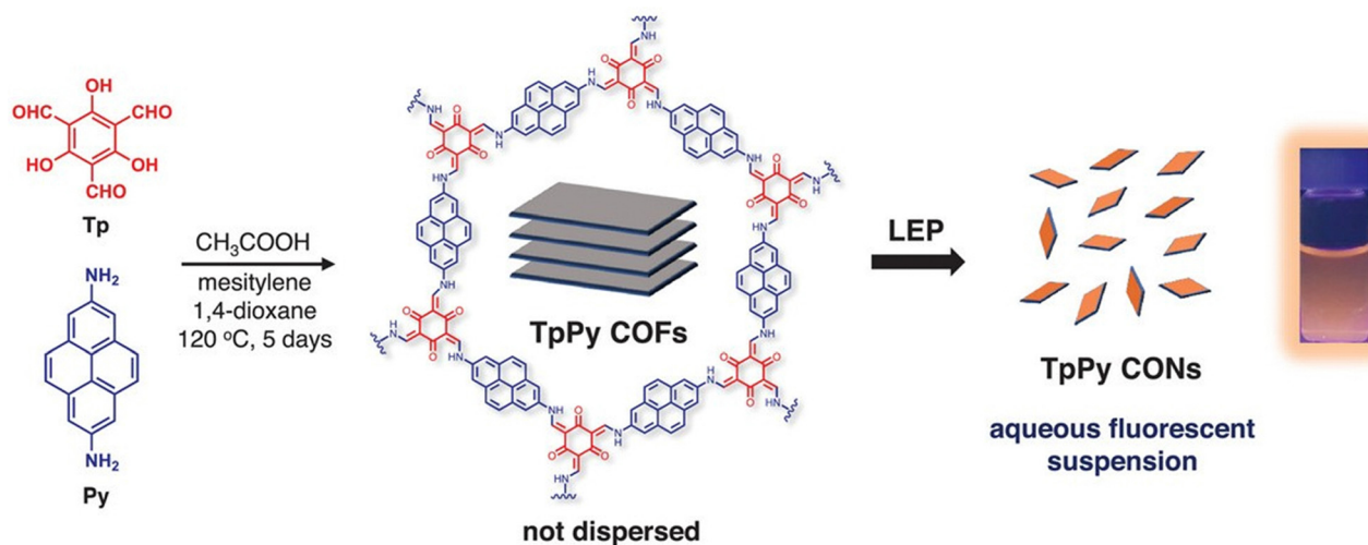
Fig. 2 Schematic diagram of the preparation of TpPy CONs by solvothermal condensation and liquid exfoliation process (fluorescent photograph of a 0.5 mg mL -1 TpPy CON dispersion taken under 365 nm UV light). Adapted with permission from ref.79.
