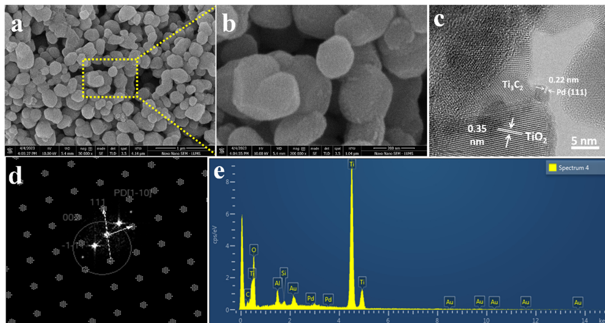
Fig. 4 SEM images at (a) 1 μm and (b) 200 nm, (c) HR-TEM, (d) TEM diffraction pattern, and (e) EDX analysis of Pd@Ti 3 C 2 T x -TiO 2 .
