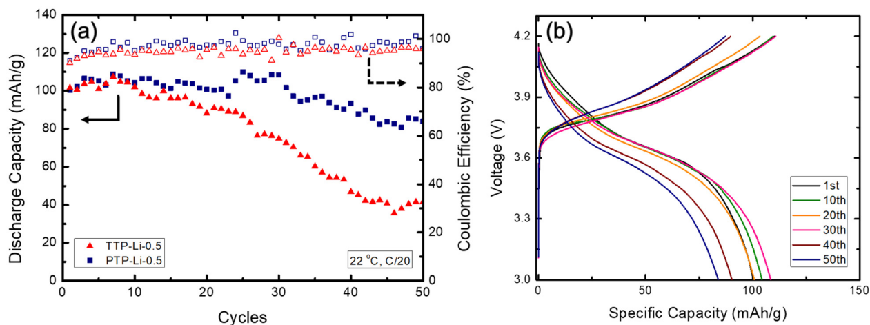
Fig. 11 (a) Discharge capacity and coulombic efficiency of Li/NMC811 cell with TTP-Li-0.5 and PTP-Li-0.5 SPEs at 22 °C cycled at C/20 and (b) selected charge and discharge profiles of Li/NMC811 cell with PTP-Li-0.5 SPE at different cycles.
