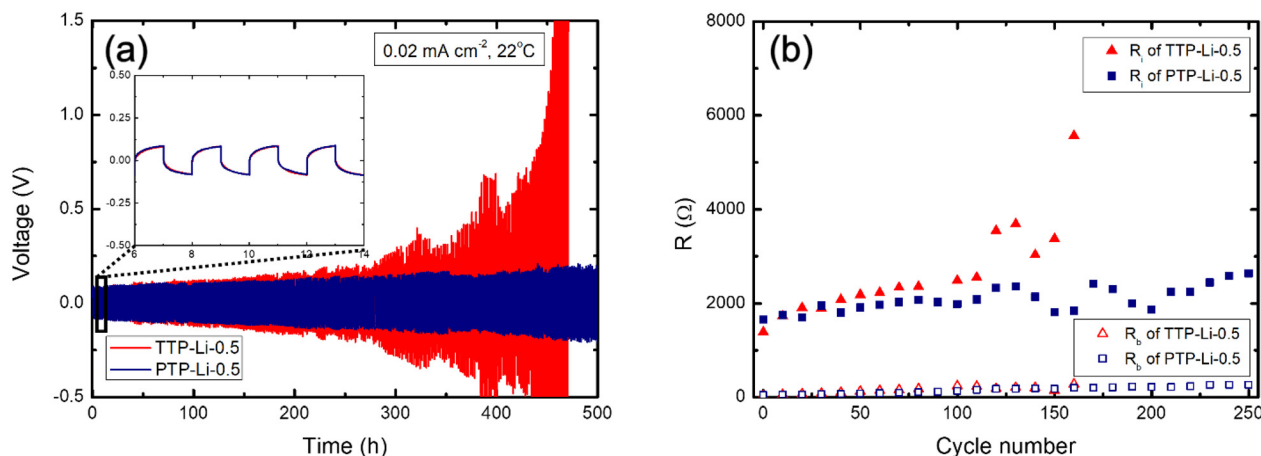
Fig. 10 (a) Stripping/plating voltage profiles of symmetric Li/SPE/Li cells cycled with the TTP-Li-0.5 and PTP-Li-0.5 SPEs under 0.02 mA cm -2 at room temperature and (b) resistances at selected cycles for the TTP-Li-0.5 and PTP-Li-0.5 SPEs.
