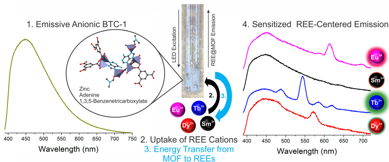
Scheme 1 Mechanism of REE detection. A blue-emitting anionic metal–organic framework, BTC-1, is immobilized on a fiber optic cable and subjected to 275 nm excitation (1). REE cations in solution are then absorbed by BTC-1 MOF (2), and excited state energy is transferred from the MOF to the encapsulated REEs (3). This sensitization process produces narrow REE-centered emission bands that are unique to each REE.
