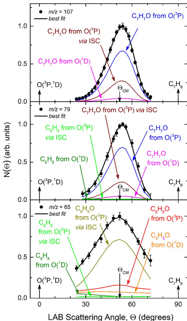
Fig. 3 LAB product angular distributions, N(\theta) , for the O(^3P,^1D) + C_7H_8 reactions at E_c = 34.7 \text{ kJ mol}^{-1} , for m/z = 107, 79 , and 65 . The partial contributions of different products at the three different masses are indicated. The black line superimposed on the experimental data corresponds to the global best-fit calculated using the CM functions shown in Fig. 6. The distinct contributions to the calculated global N(\theta) are color-coded as in Fig. 2, and indicated with the formula of the corresponding product.
