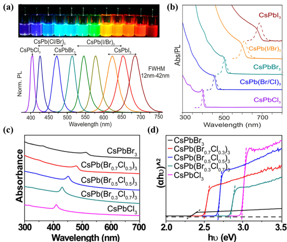
Fig. 4 (a) Colloidal halide perovskite \text{CsPbX}_3 NCs ( X = \text{Cl}, \text{Br}, \text{and I} ) exhibit size- and composition-tunable bandgap energies covering the entire visible spectral region with narrow and bright emission. 64 (b) Typical optical absorption and PL spectra of \text{CsPbX}_3 NCs. 64 (c) UV-vis absorption spectra and (d) (\alpha h\nu)^2 versus h\nu curves of \text{CsPb}(\text{Br}_x/\text{Cl}_{1-x})_3 ( x = 1, 0.7, 0.5, 0.3, 0 ) materials. 65
