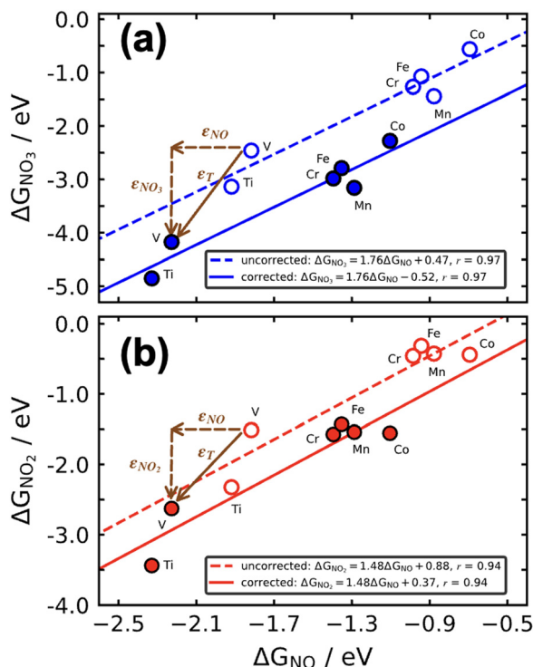
Fig. 15 Free energies of adsorption of ^*NO_3 (a) and ^*NO_2 (b) versus that of ^*NO on metallocporphyrins. Dashed lines and open circles correspond to uncorrected energies, solid lines and solid circles correspond to energies upon gas-phase corrections. Brown vectors on the V-containing porphyrin show the displacements introduced by the respective gas-phase errors. Reproduced from ref. 29, licensed under CC BY 4.0 ( https://creativecommons.org/licenses/by/4.0/ ).
