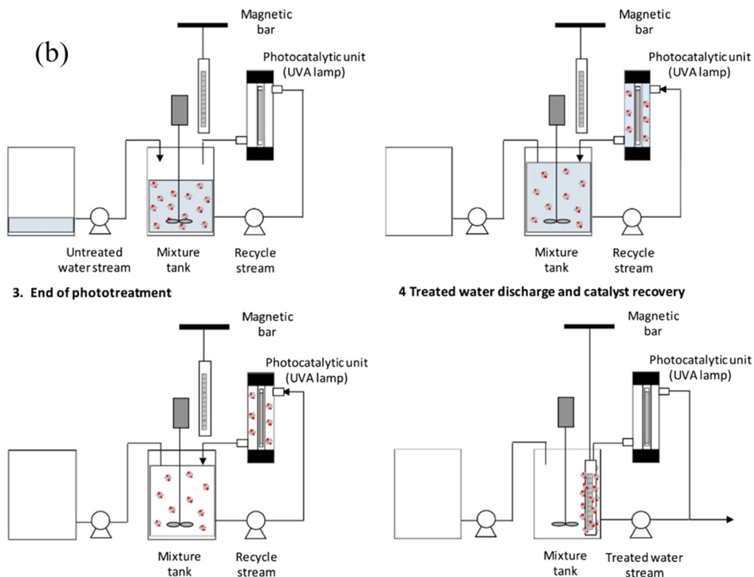
Fig. 8 (a) Challenges of MRNPCs in practical applications; (b) operation of magnetic photocatalytic reactor: 1) loading of MRNPCs and water, 2) continuous phototreatment; 3) end of phototreatment, 4) MRNPCs recycling. Reproduced from ref. 70 with permission from Elsevier, copyright 2019.
