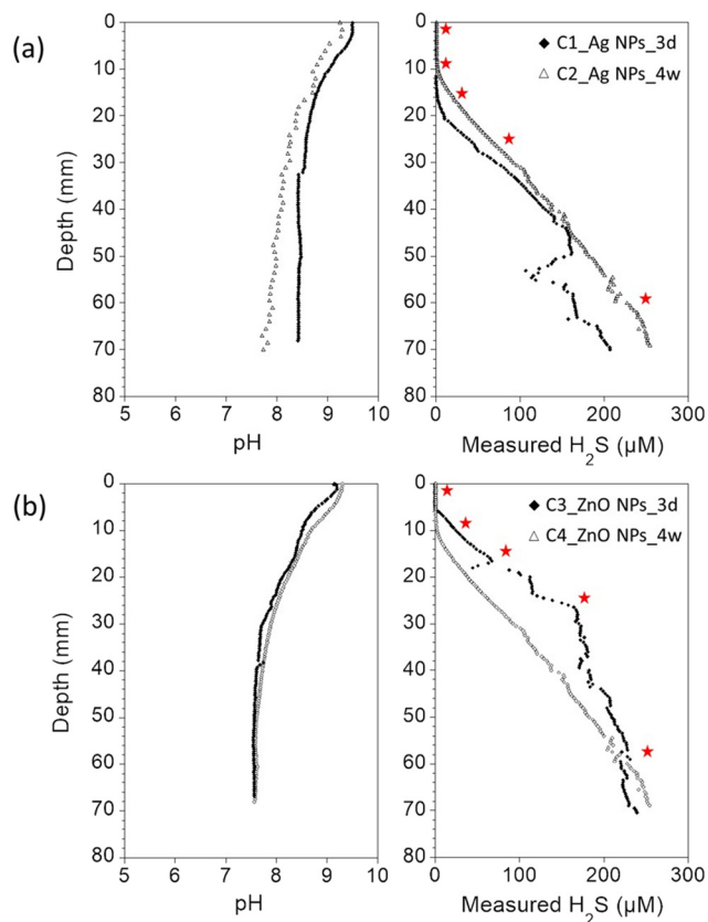
Fig. 3 Pore water depth profiles of pH and measured H 2 S concentration in the incubated sediment cores used to expose (a) Ag NPs and (b) ZnO NPs-TEM grids. The red stars correspond to the depths at which the NPs-TEM grids were inserted in the sediment columns.
