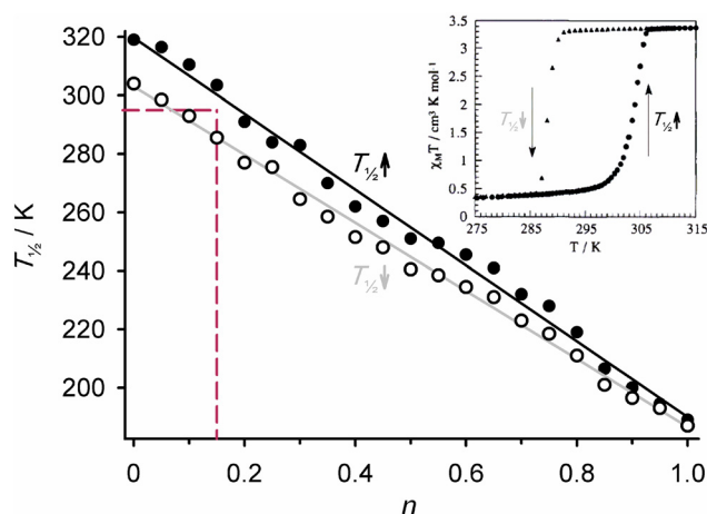
Fig. 7 Measured (circles) and calculated (lines) dependence of T_{1/2} on composition in [\text{Fe}(\mu\text{-atz})_z(\mu\text{-Htrz})_{3-3n}][\text{ClO}_4]_2 \cdot \text{H}_2\text{O} . The dashed lines indicate the composition z that is thermally bistable at room temperature (magnetic data shown in inset). The data were replotted from ref. 132, while the inset is adapted from ref. 134 with permission from Springer/Nature, copyright 2009.
