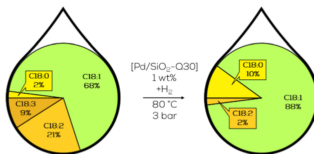
Fig. 21 C18 fatty acid composition in the hydrogenation of canola oil-derived biodiesel over macroporous Pd on SiO 2 as performed by Luengnaruemitchai. 127
