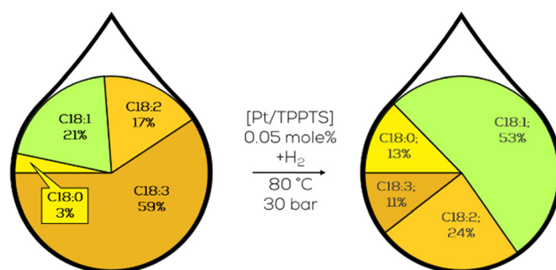
Fig. 36 Fatty acid composition of the C18 fraction in the partial hydrogenation of linseed oil-derived methyl ester as performed by Papadogianakis. 189
