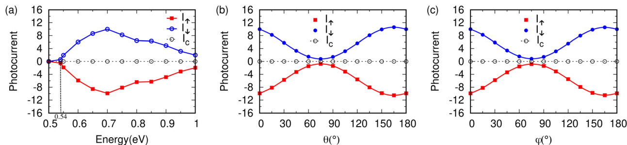
Fig. 3 The spin-up I_\uparrow and spin-down I_\downarrow photocurrent, and total charge photocurrent I_c as a function of: (a) photon energy under LPL with a polarization angle \theta = 0^\circ ; (b) polarization angle \theta under LPL with photon energy \hbar\omega = 0.70 eV; (c) helicity angle \phi under EPL with \hbar\omega = 0.70 eV. In the EPL case, \phi = 45^\circ and 135^\circ mean right and left circularly polarized light, respectively. " I_\uparrow ", " I_\downarrow " and " I_c " mean the spin up, spin down and total charge photocurrent, respectively.
