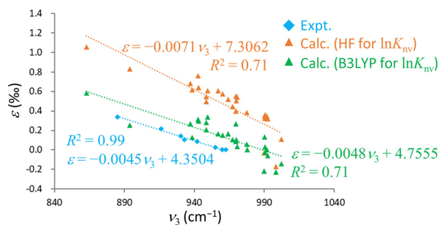
Fig. 4 Relationships between \nu_3 and \varepsilon . The horizontal axis shows \nu_3 in units of cm^{-1} while the vertical axis shows \varepsilon in units of ‰. The dotted lines are linear regressions and r^2 is the coefficient of determination in each case.
