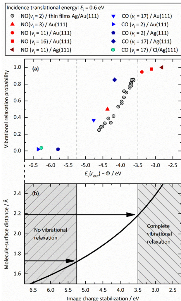
Fig. 12 (a) Relaxation probability of various molecule-surface systems as a function of E_v - \Phi at an incidence translational energy of 0.6 eV. The results are shown for CO ( v_i = 17 )/Ag(111), CO ( v_i = 17 )/Au(111), CO ( v_i = 2 )/Ag(111), CO ( v_i = 2 )/Au(111), NO ( v_i = 11 )/Ag(111), NO ( v_i = 3, 11, 16 )/Au(111), and NO ( v_i = 2 ) on thin films of Ag on Au(111). All systems follow a common trend showing an increase of the relaxation probability from 0 to 1 between -5.25 eV and -3.5 eV (b) Image charge stabilization (ICS) of a negatively charged molecule in the vicinity of the surface. The ICS must compensate for the difference E_v(r_{out}) - \Phi to make the ET energetically feasible. Little vibrational relaxation occurs for ICS values below -5.25 eV as the molecule cannot get closer to the surface and approaches the repulsive wall at which it is scattered back. For values above -3.5 eV, the molecule remains long enough in regions of electronic non-adiabaticity so that complete vibrational relaxation occurs. The arrows indicate corresponding molecule-surface distances. Reproduced from ref. 64 with permission from the PCCP Owner Societies.
