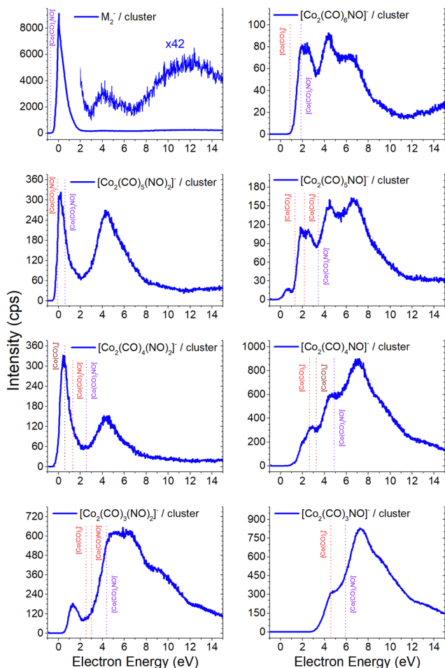
Fig. 2 The molecular dimer [\text{M}_2]^- and the associated smaller clusters formed via CO and/or NO ligand losses obtained from CLUSTER-ILN measurements and compared with the calculated CBS-QB3 reaction energies of the suggested [ion + neutral] product pair (dashed lines with violet for \text{M}^- accounted in the [ion + neutral] pair, with red for the typical DEA fragment of \text{M}^- in the pair, and with wine for rearrangement products like [\text{Co}(\text{CO})_4]^- ).
