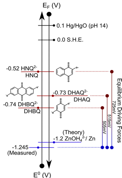
Fig. 1 Electrode potential scale showing the location of the approximate redox potentials both versus a standard reference ( E^0 ) and absolute electron energy ( E_r ), for both the zinc/zincate couple and quinone redox couples selected as mediators. Equilibrium overpotentials between the liquid/solid components are indicated on the right-hand side. Please see ESI† for complete compound names and discussion of reactions.
