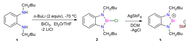
Scheme 1 Syntheses of complexes 2–3 .
