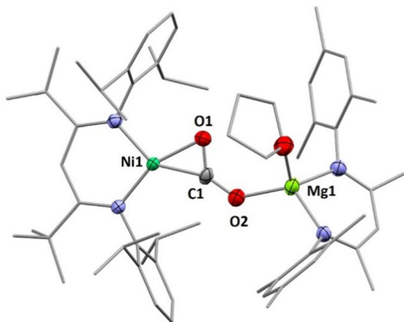
Fig. 3 Molecular structure of 3 . H atoms and co-crystallised solvent molecules omitted for clarity. Selected bond lengths (Å) and angles (°): Ni1–C1 1.839(2), Ni1–O1 1.925(2), C1–O1 1.269(4), C1–O2 1.236(3), O1–C1–O2 129.3(3), O2–Mg1 1.974(2).
