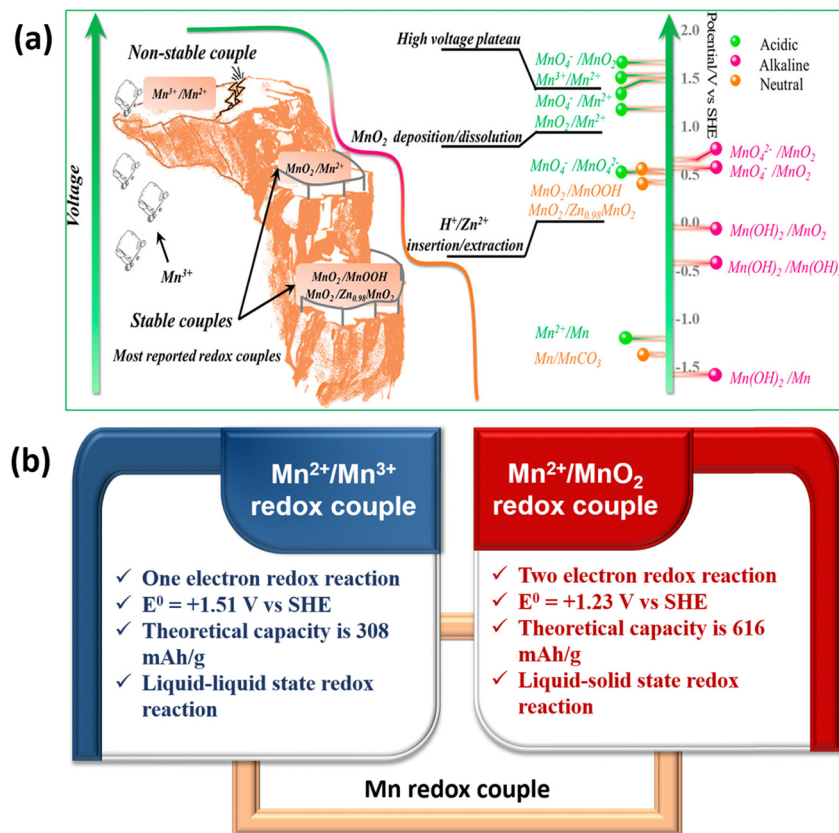
Fig. 4 (a) Schematic illustration of manganese redox couples in different electrolytes (reproduced from ref. 43 with permission from the American Chemical Society) and (b) comparison of Mn²⁺/Mn³⁺ and Mn²⁺/MnO₂ redox couple characteristics.
