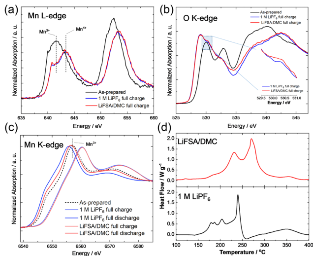
Fig. 3 (a and b) Soft and (c) hard XAS spectra of nanosized \text{Li}_{1.14-y}\text{Ti}_{0.29}\text{Mn}_{0.57}\text{O}_2 on charge/discharges. (d) DSC curves of charged nanosized \text{Li}_{1.14-y}\text{Ti}_{0.29}\text{Mn}_{0.57}\text{O}_2 with different electrolyte solutions.
