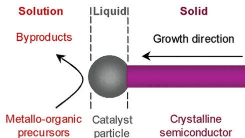
Fig. 2 The reaction mechanism of the SLS method. Reproduced with permission from ref. 27. Copyright 2006 American Chemical Society.
