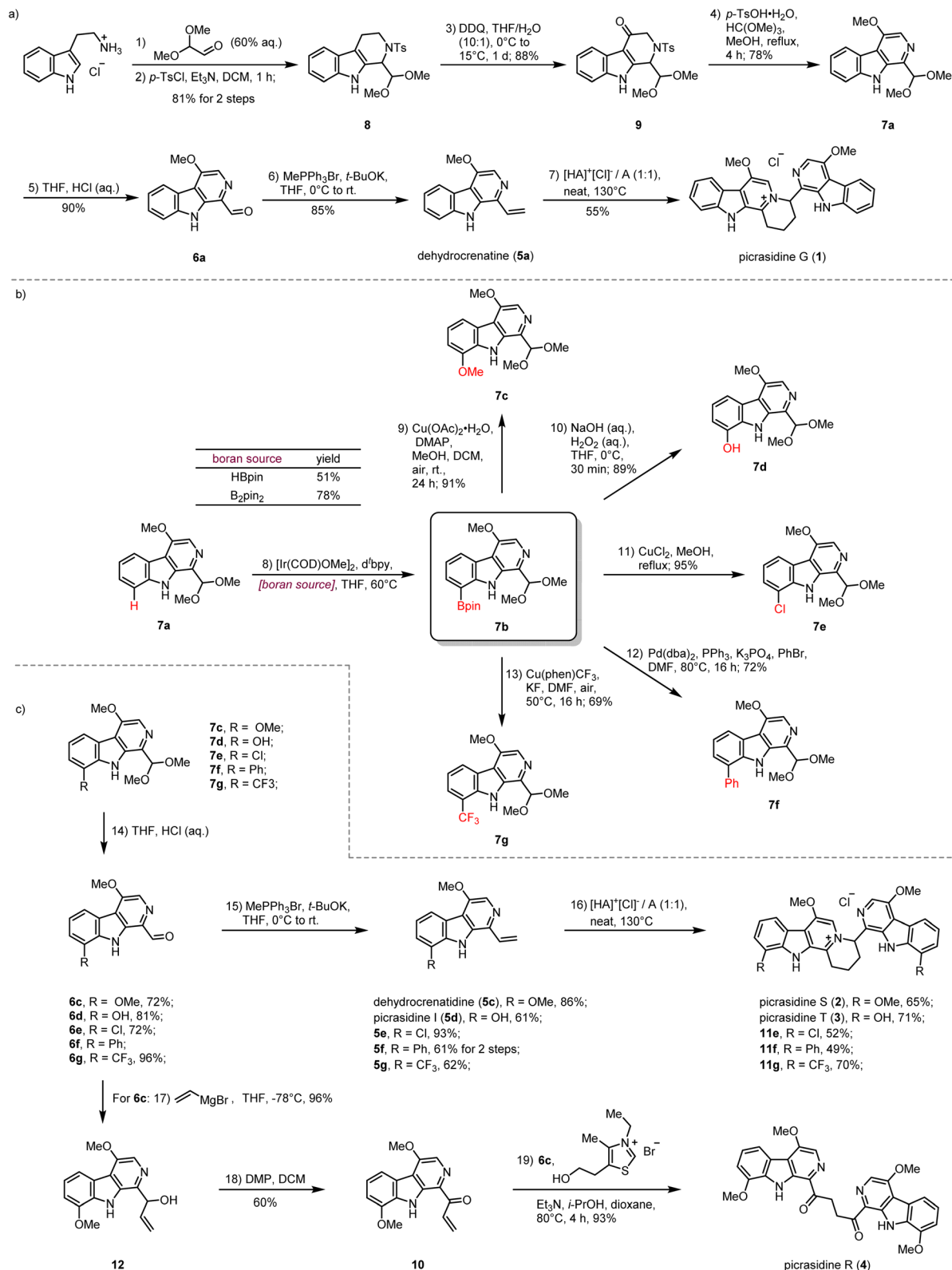
Scheme 2 (a) Syntheses of picrasidines G (1) by the aza-[4 + 2] cycloaddition. (b) Late-stage C–H functionalization strategy for diversity-oriented syntheses of C-8 substituted β-carboline alkaloids. (c) Total syntheses of picrasidines S (2), T (3), R (4) and 11e, 11f, 11g.
