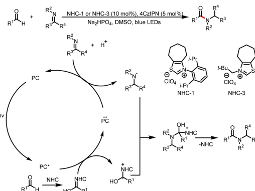
Scheme 5 Amide synthesis from aldehydes and imines.
