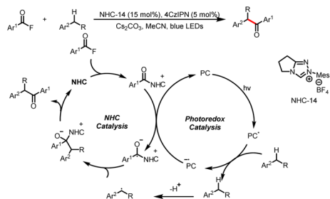
Scheme 34 Construction of benzyl aryl ketones by benzylic \text{C}(\text{sp}^3) -arylation.
