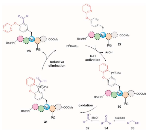
Fig. 8 Proposed mechanism for the Pd-catalyzed ortho -acetylation of peptides.
