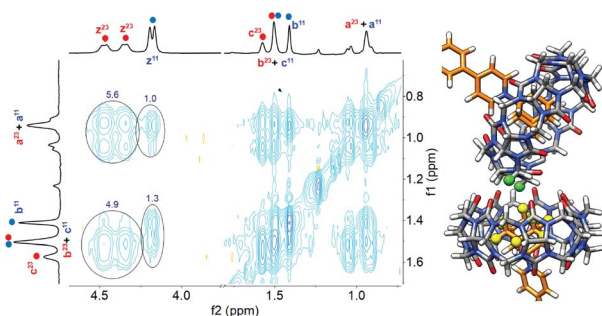
Fig. 3 1 H– 1 H NOESY spectrum of a 1:1 mixture of complex CB[7]·1 and putative aggregate (CB[7] \cdot 1)_3Na . The correlations between adamantyl signals H a and H b with equatorial methylenes H x at the CB[7] portals are highlighted. Section of an optimized structure of putative complex (CB[7] \cdot 1)_3Na , with interacting hydrogens H x highlighted in green, and H a and H b in yellow.
