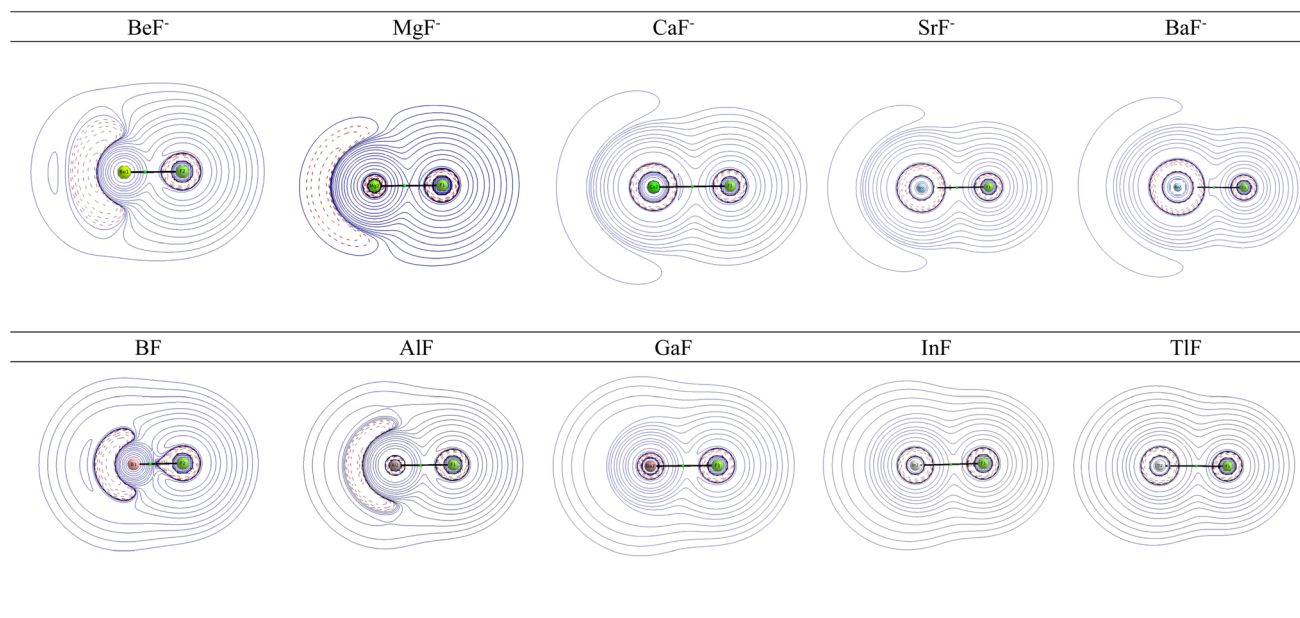
Fig. 2 Laplacian distribution \nabla^2\rho(r) of \text{AeF}^- ( \text{Ae} = \text{Be} - \text{Ba} ) and \text{EF} ( \text{E} = \text{B} - \text{Tl} ) at the CCSD(T)/def2-TZVPP level. Red lines indicate the areas of charge concentration ( \nabla^2\rho(r) < 0 ), while blue lines show the areas of charge depletion ( \nabla^2\rho(r) > 0 ). The solid lines connecting the atomic nuclei are the bond paths. Green dots are bond critical points.
