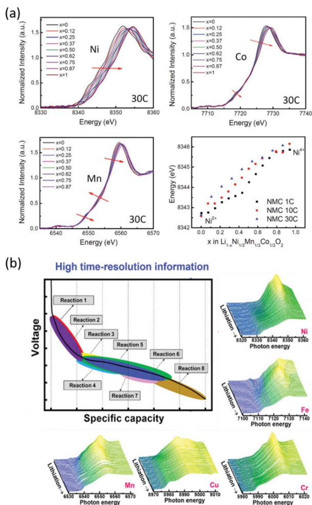
Fig. 4 Two examples of operando quick-scanning XAS: (a) XANES results of \text{LiNi}_{0.33}\text{Mn}_{0.33}\text{Co}_{0.33}\text{O}_2 at Ni, Co, and Mn K-edges throughout oxidation at a 30C rate. Reproduced from ref. 75 with permission ©John Wiley&Sons. (b) Voltage vs. capacity profile for the (\text{CrMnFeNiCu})_3\text{O}_4 HEO electrode, and corresponding XAS spectra which enable changes in the oxidation state/coordination for the involved metal ions to be inferred as a function of the electrode state of charge. 76
