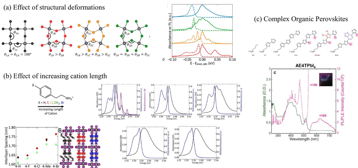
Fig. 6 (a) The exciton fine structure in the UV-vis absorption and emission spectrum in perovskites changes as a function of structural deformation 153 or (b) increasing length of the organic cations. 297 (c) Vibronic progression observed in the UV-vis absorption spectrum of (\text{AE4T})\text{PbI}_4 . 298 (a) Reprinted with permission from ref. 153. Copyright 2020 American Chemical Society. (b) Reprinted with permission from ref. 297. Copyright 2019 American Chemical Society.
