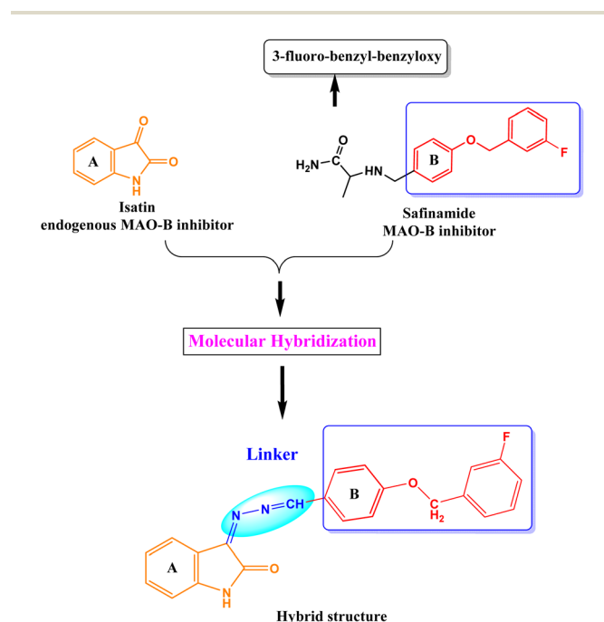
Fig. 1 Design strategy of benzyloxy isatin hydrazones.
