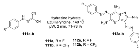
Scheme 39 Synthesis of diarylo-2,5,7-triaminopyrazolo[1,5- a ]pyrimidines 112a–b .
