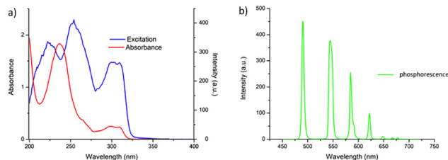
Fig. 3 (a) The UV-vis absorption (red) and excitation spectra ( \lambda_{\text{em}} = 545 \text{ nm} ) of the btp complex 3.Tb in \text{CH}_3\text{CN} showing sensitisation arising from ligand-centred energy transfer (left), and time-gated emission spectrum of 3.Tb showing the characteristic \text{Tb(III)} centred-emission.
